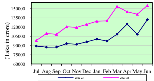
Fig. 20: MFS TRANSACTIONS
